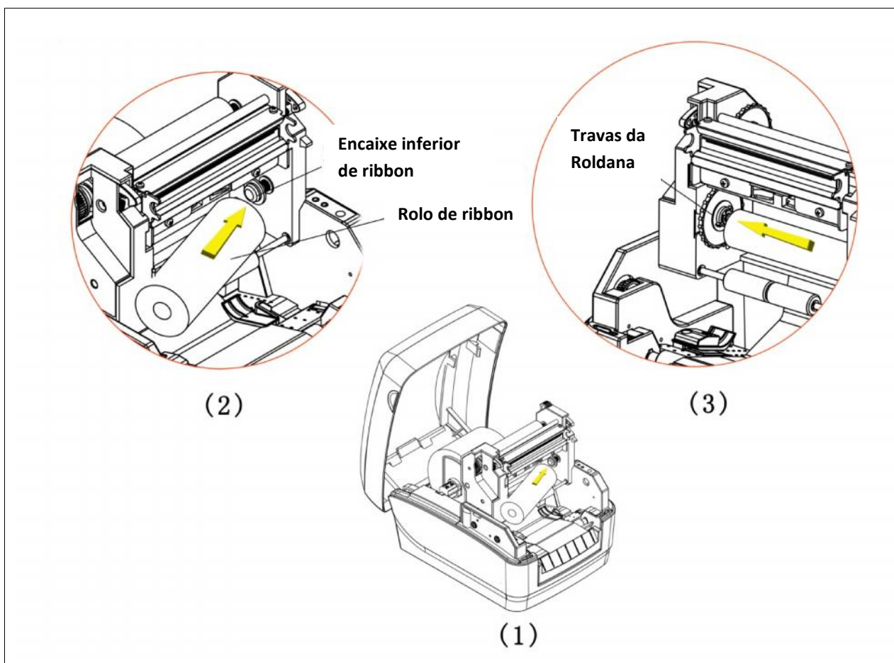
Fig. 13 – Instalando o rolo de ribbon
